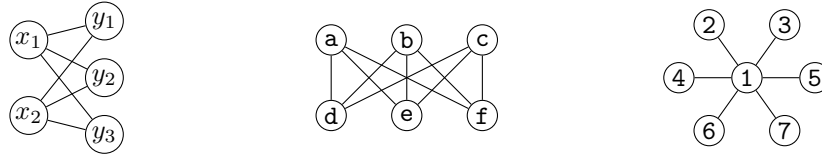
Figure 5: The bipartite graphs K_{2,3}, K_{3,3} and K_{1,6} .
