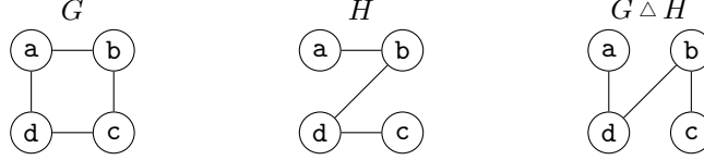
Figure 9: Symmetric difference of two graphs.
