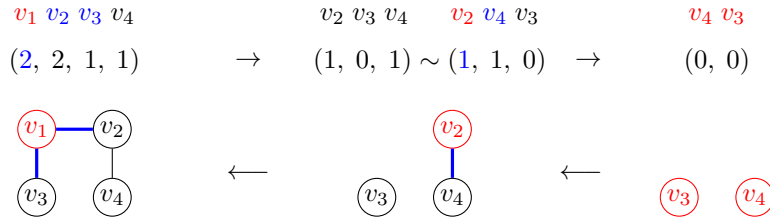
Figure 13: Realising a graph from a graphic sequence.
