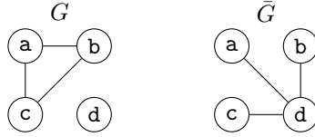
Figure 7: A graph and its complement.
