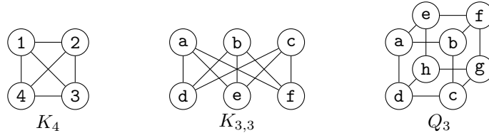
Figure 12: Three cubic graphs.
