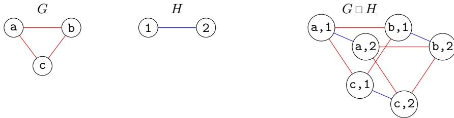
Figure 8: Cartesian product of two graphs.
