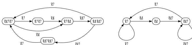
Figure 4.1: The Rauzy graphs G_2(S) and G_1(S) for the decoding of the Fibonacci set into blocks of length 2.
