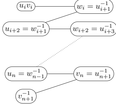
Figure 5.4: The graph G(X) .
