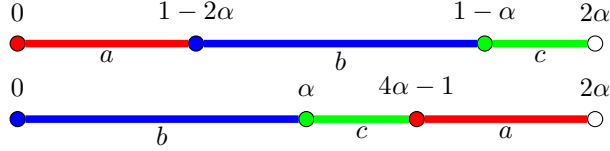
Figure 5: The transformation induced on I .
