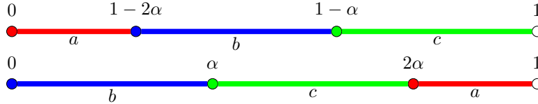
Figure 3: A 3-interval exchange transformation.
