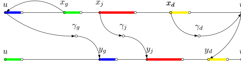
Figure 7: The transformation induced on [u, v[ .
