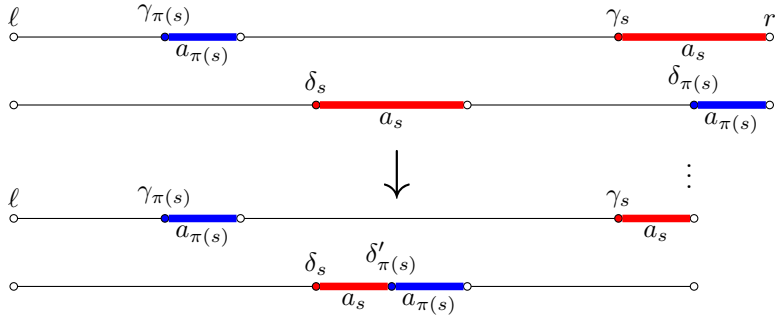
Figure 8: Case 0 in Rauzy induction.
