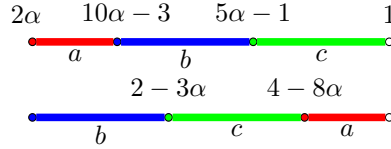
Figure 11: The transformation S .
