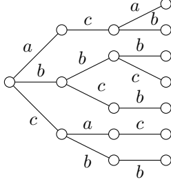
Figure 2: The words of length \leq 3 of \mathcal{D}_f(F) .
