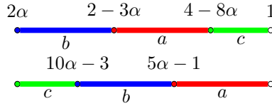
Figure 12: The transformation U .
