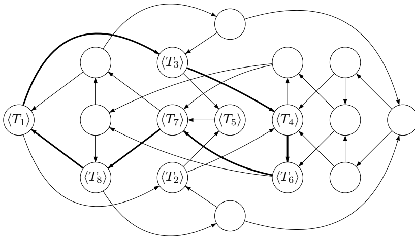
Figure 15: Modified induction graph of the transformation T .
