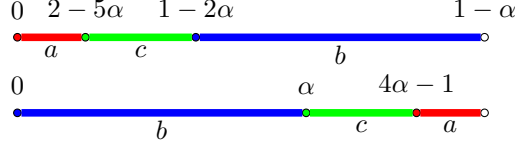
Figure 10: The transformation \psi^2(T) .
