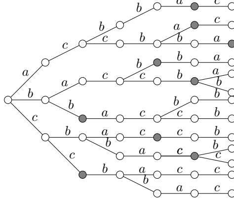
Figure 1: The words of length \leq 6 of the set F .
