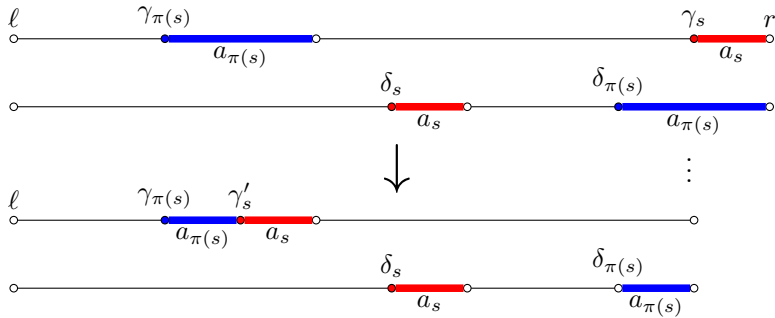
Figure 9: Case 1 in Rauzy induction.
